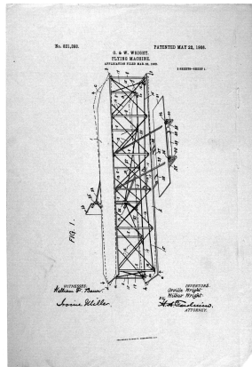
Figure 5. Diagram from the Wright brothers' patent application for a "flying machine," filed March 23, 1903.
